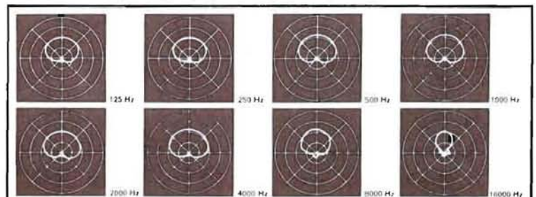
Polar diagrams (photographs), taken from 1 m distance from the source of sound. Directional characteristic: Position "Cardioid"
